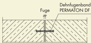
Dehnfuge in Bodenplatte
